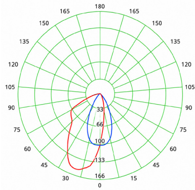
SNAP Uni 2.0 beam
