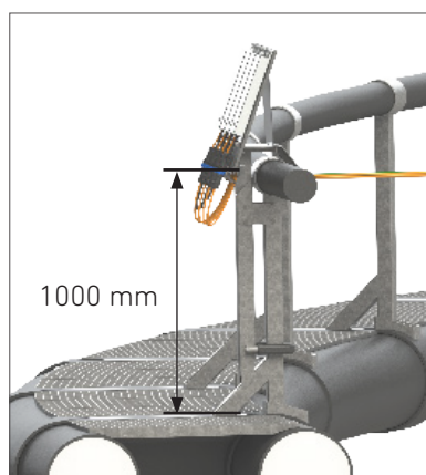
Aqualine, universell brakettmontering
