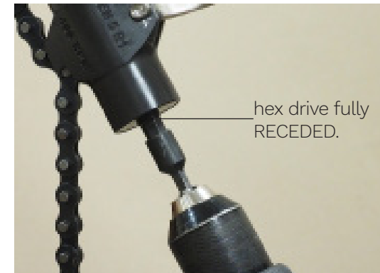
Fig. 8.2 STOP drilling once the hex drive has fully receded inside the Drill Jig.
