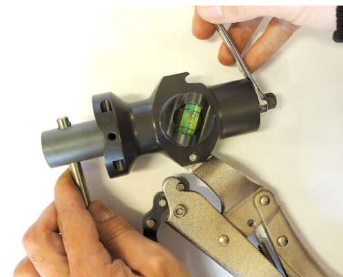
Fig. 3.4 Use the cutter removal tool and spanner provided to remove or secure the cutters. Note the cutter removal tool's 15mm side (shallow) and 16mm side (deep).
