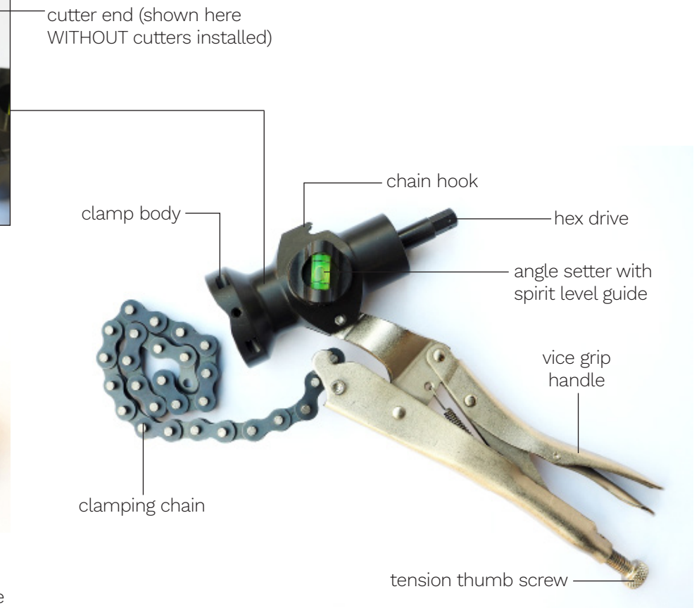
G5 Drill Jig Parts
