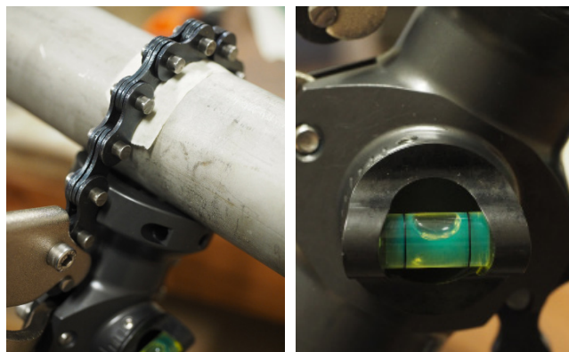
Fig. 6.2 - 6.5 align clamp body with the tape and engage the chain hook and clamping chain. Ensure the spirit level bubble remains centred planetlighting.com/led-puck
