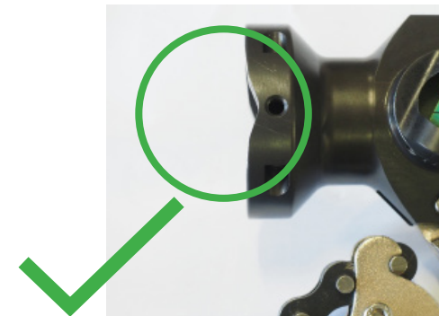
CORRECT. Cutters are installed and fully retracted inside the cutter assembly.
