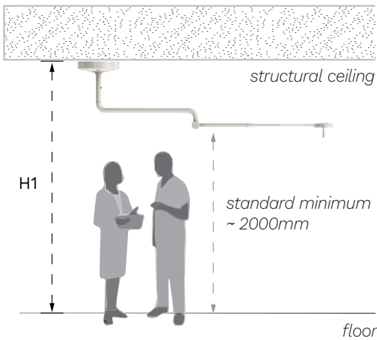
Direct Ceiling Mount
