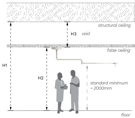
False Ceiling Mount
