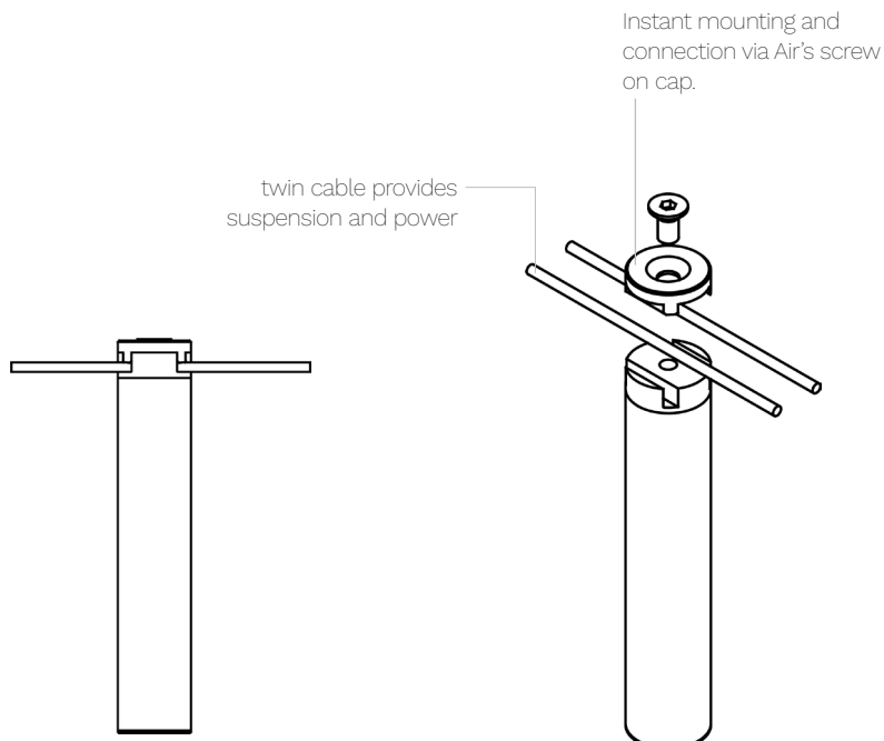
Luminaire connected (cap on) Side view
