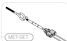
Metal Mount Set For metal surfaces
