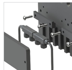
2 x 2-outlet plug board
